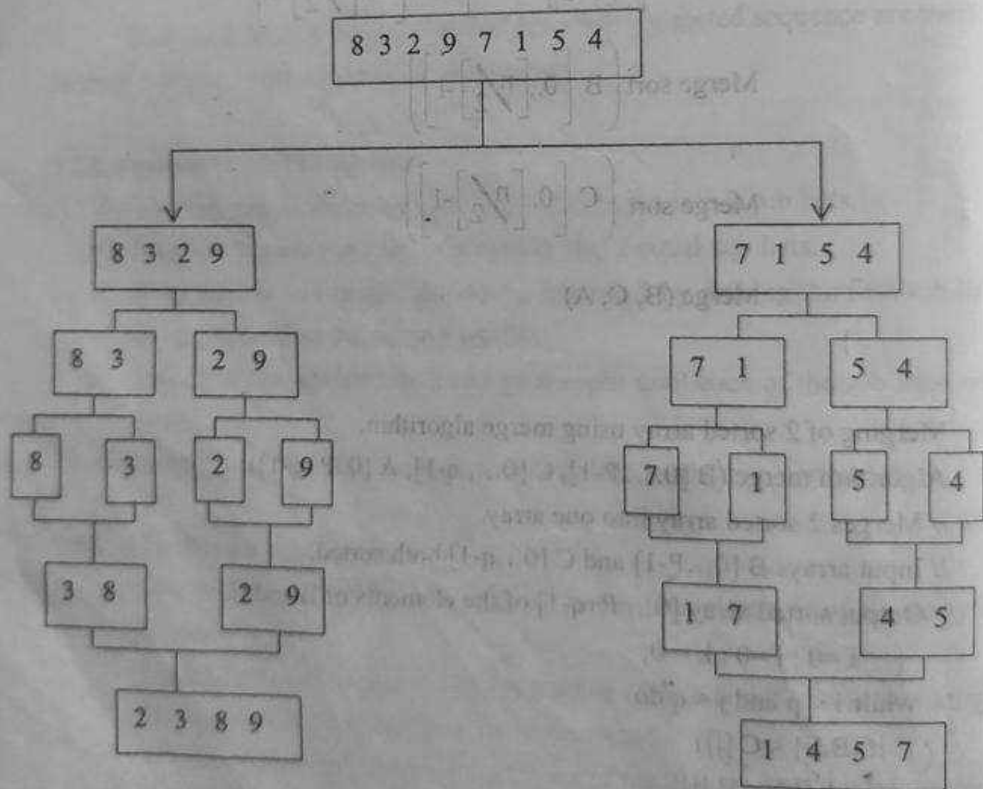
Fig 2.2 Merge sort.
